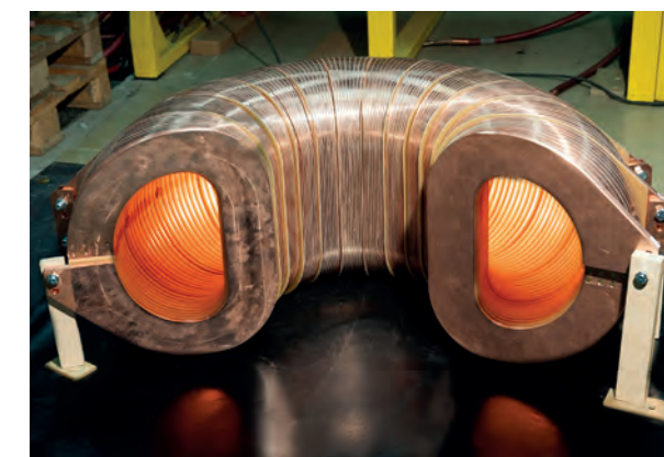
Fig. 2: Inductive storage device developed at ISL. The toroidal coil can store 1 MJ and is designed to power railguns
