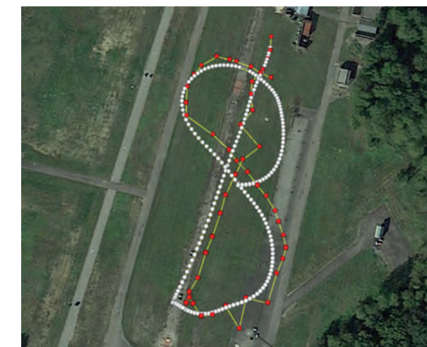
Fig. 2: Tracking of a small UAV using three acoustic arrays ("8 shape trajectory"). White points: ground real data, red points: estimated position
