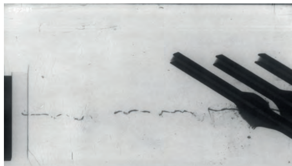
Shaped charge jet disturbed by bulging armour plates
