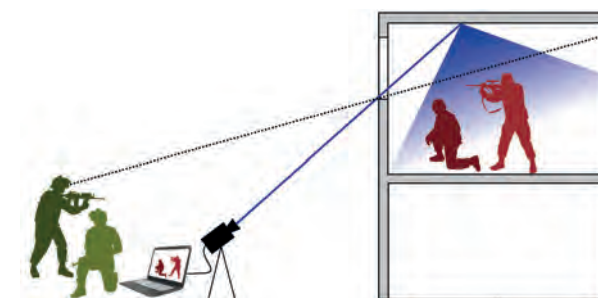
Non-line of sight imaging could be used in urban environment to identify alien forces in hideouts
