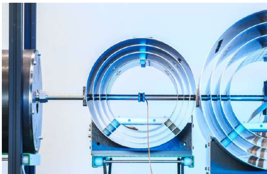
In the magnetic flow measurement process, a strong magnet polarizes the fluid, which flows from left to right through the structure in a steel pipe. The central screen contains the HF coil, which implants the marker in the fluid. A quantum sensor in the right screen detects the marker.
